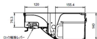
B-B (1:5)
